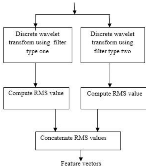
Fig.1 Generation of Feature Vector
