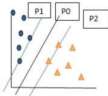
Fig.3 Support vectors and hyper plane.
